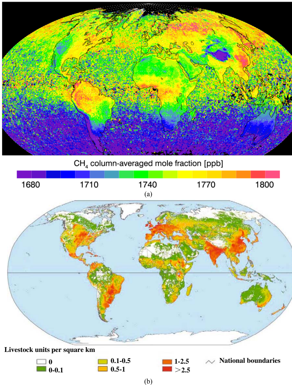
Fig. 5 (a) Global atmospheric methane distribution as measured by the ENVISAT satellite over three complete years, 2003-2005 [69, 70]; (b) Global total livestock distribution of both ruminants and monogastrics [1]. There is no discernible geographical relationship between methane and livestock distribution.
